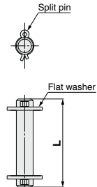
Clevis pin/Knuckle joint pin
