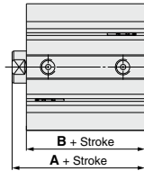
Double acting, Single rod/Large bore
