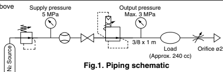
Fig. 1. Piping schematic
