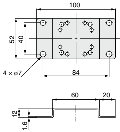
Flat bracket
