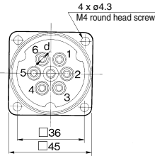
Panel mounting hole
