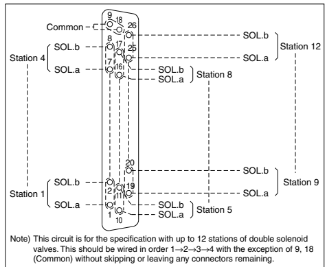
Type FB: D-sub connector (26 pins)
