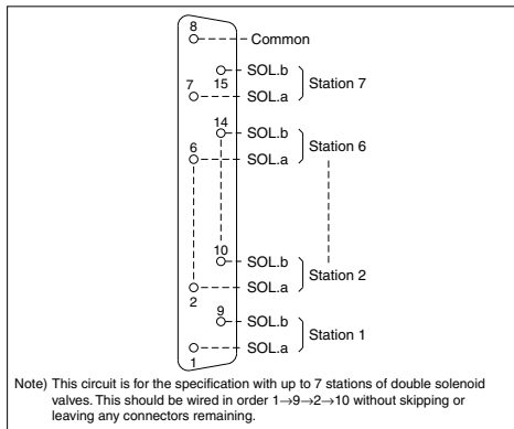
Type FA: D-sub connector (15 pins)
