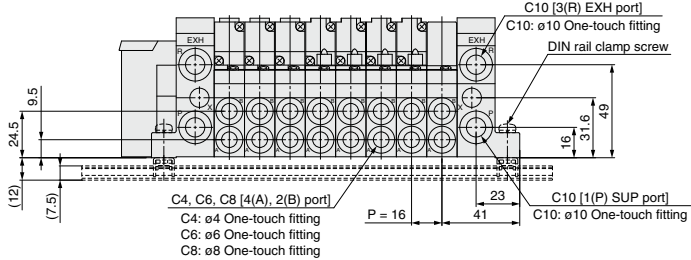
Dust-tight, Water-jet-proof SI unit: L8 = 16n + 118.5, L9 = 16n + 131 L10 = L3 + 50, L11 = L4 + 50
