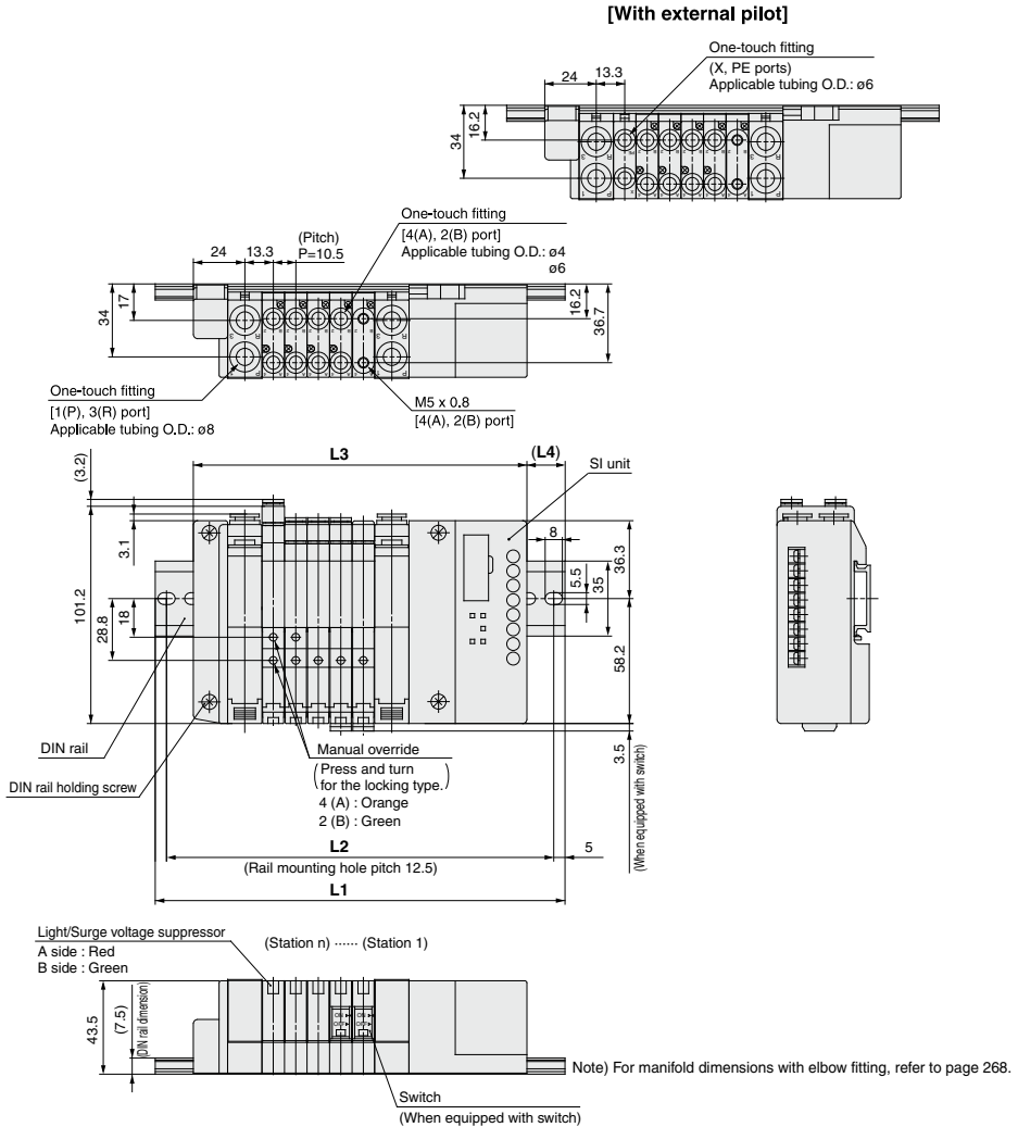
Internal Pilot Manifold L Dimension n : Stations
