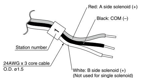
Single solenoid
