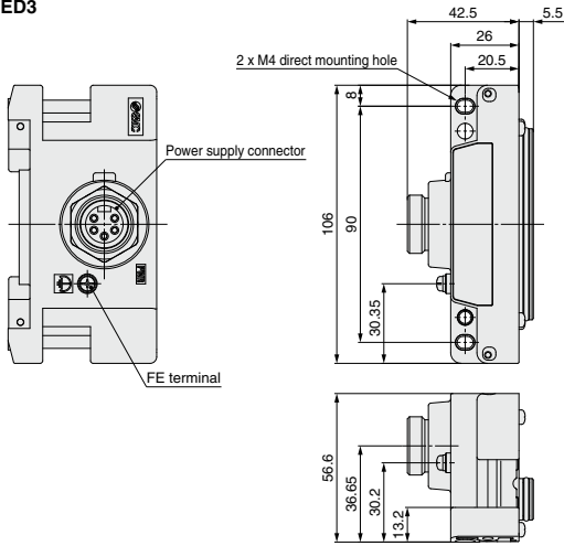
Power supply connector PWR: 7/8 inch 5-pin plug
