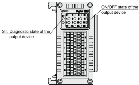
EX600-DY□F
