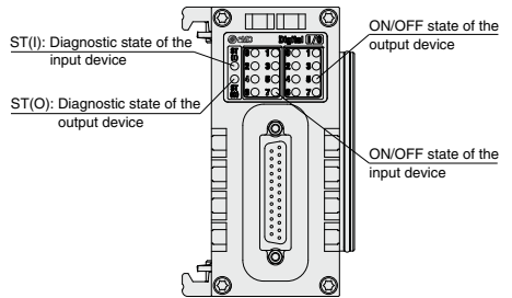
EX600-DM□E
