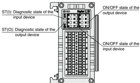
EX600-DM□F
