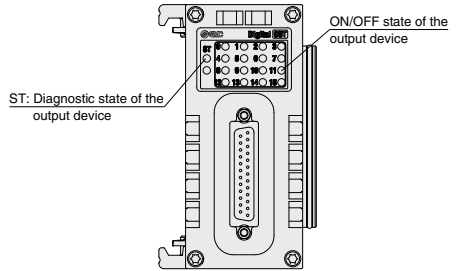
EX600-DY□E
