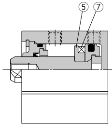
Built-in magnet
