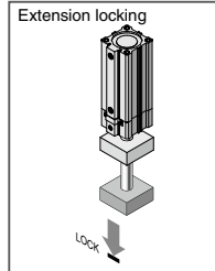
Drop prevention for press fitting attachment
