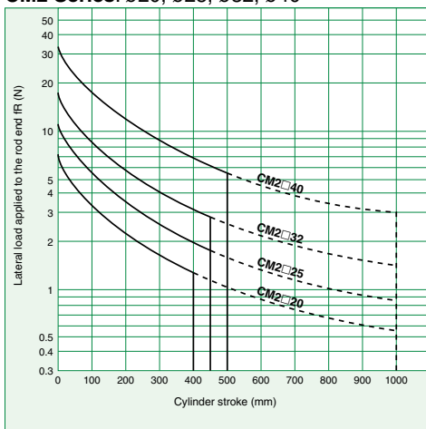
Graph (12) CM2 Series: \varnothing 20, \varnothing 25, \varnothing 32, \varnothing 40
