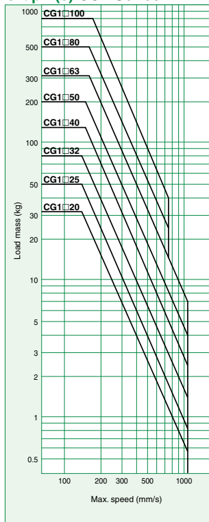
Graph (8) CG1 Series
