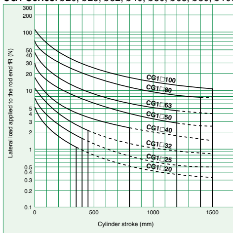
Graph (13) CG1 Series: \varnothing 20, \varnothing 25, \varnothing 32, \varnothing 40, \varnothing 50, \varnothing 63, \varnothing 80, \varnothing 100
