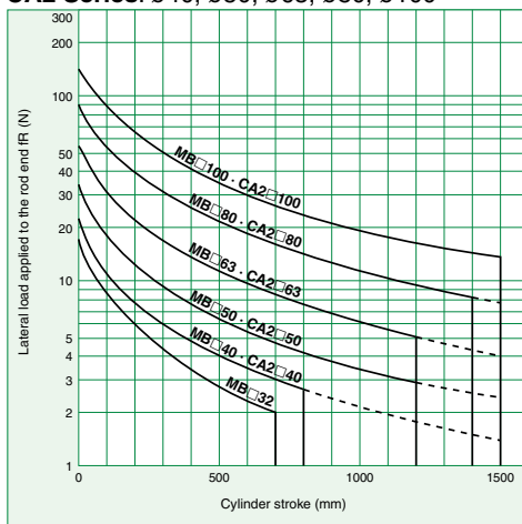
Graph (14) MB Series: \varnothing 32, \varnothing 40, \varnothing 50, \varnothing 63, \varnothing 80, \varnothing 100 CA2 Series: \varnothing 40, \varnothing 50, \varnothing 63, \varnothing 80, \varnothing 100
