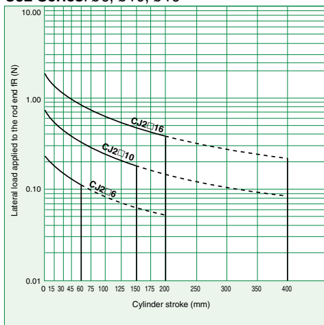
Graph (11) CJ2 Series: \varnothing 6, \varnothing 10, \varnothing 16
