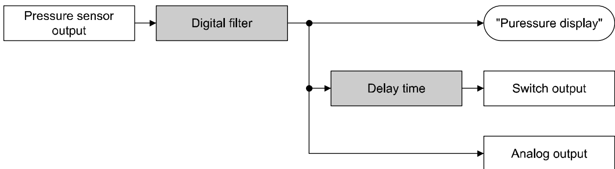
Fig.: Relation between the filter and response time
