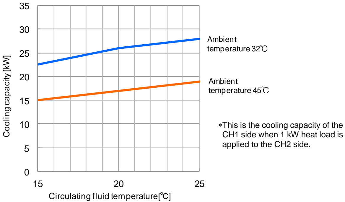
Fig. 8-7 Cooling Capacity (HRL300-A*-20)
