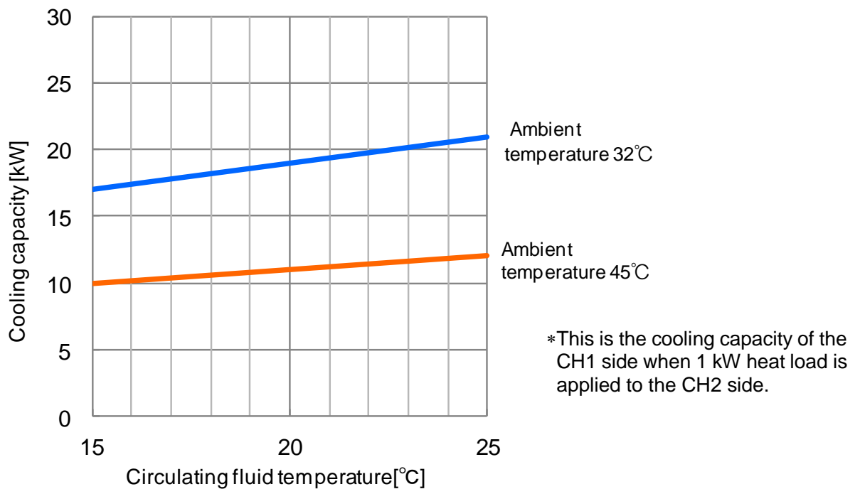
Fig. 8-6 Cooling Capacity (HRL200-A*-20)
