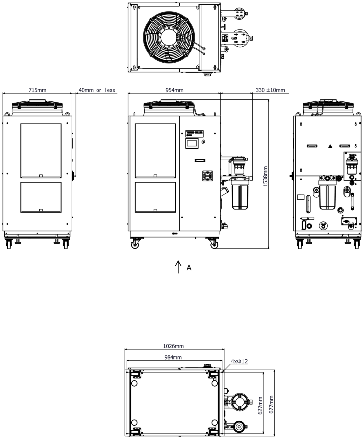
Dimensions for the positions of the anchor bolts (View A)
