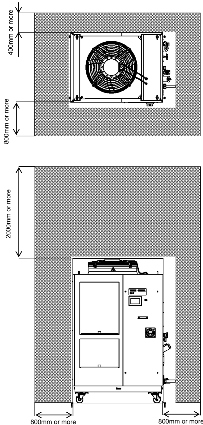
Fig. 3-3 Installation space (This drawing shows "HRL200-A-20".)
