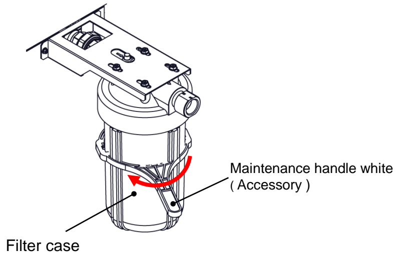
Fig. 3-15 CH1 particle filter case removal
