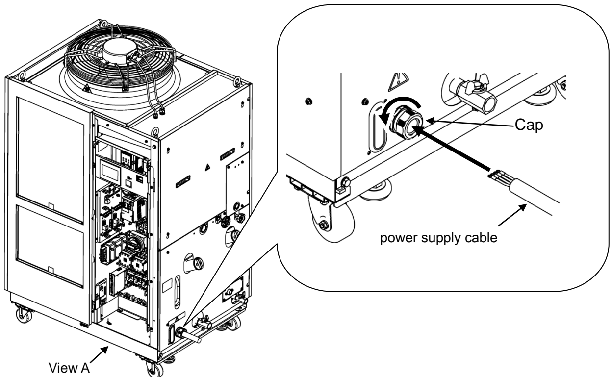
Fig. 3-8 Wiring of power supply cable
