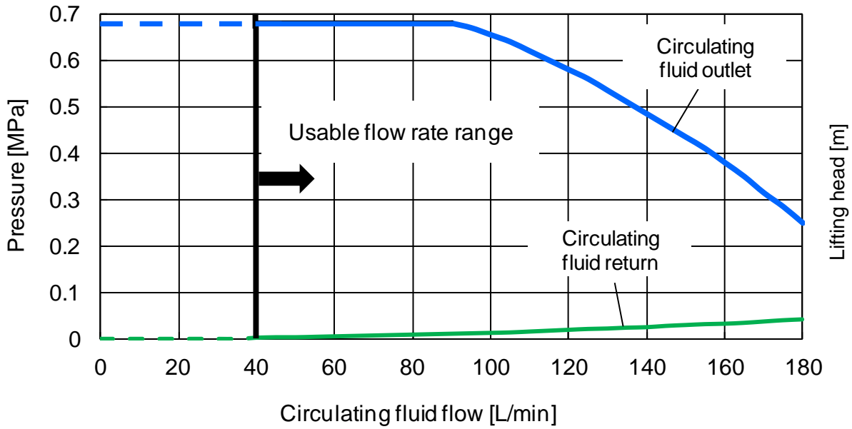
Fig. 8-11 Pump capacity(HRL300-A*-20 CH1)
