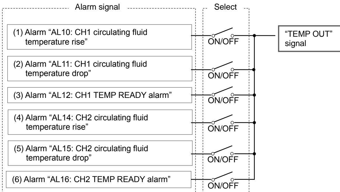
TEMP OUT signal output chart
