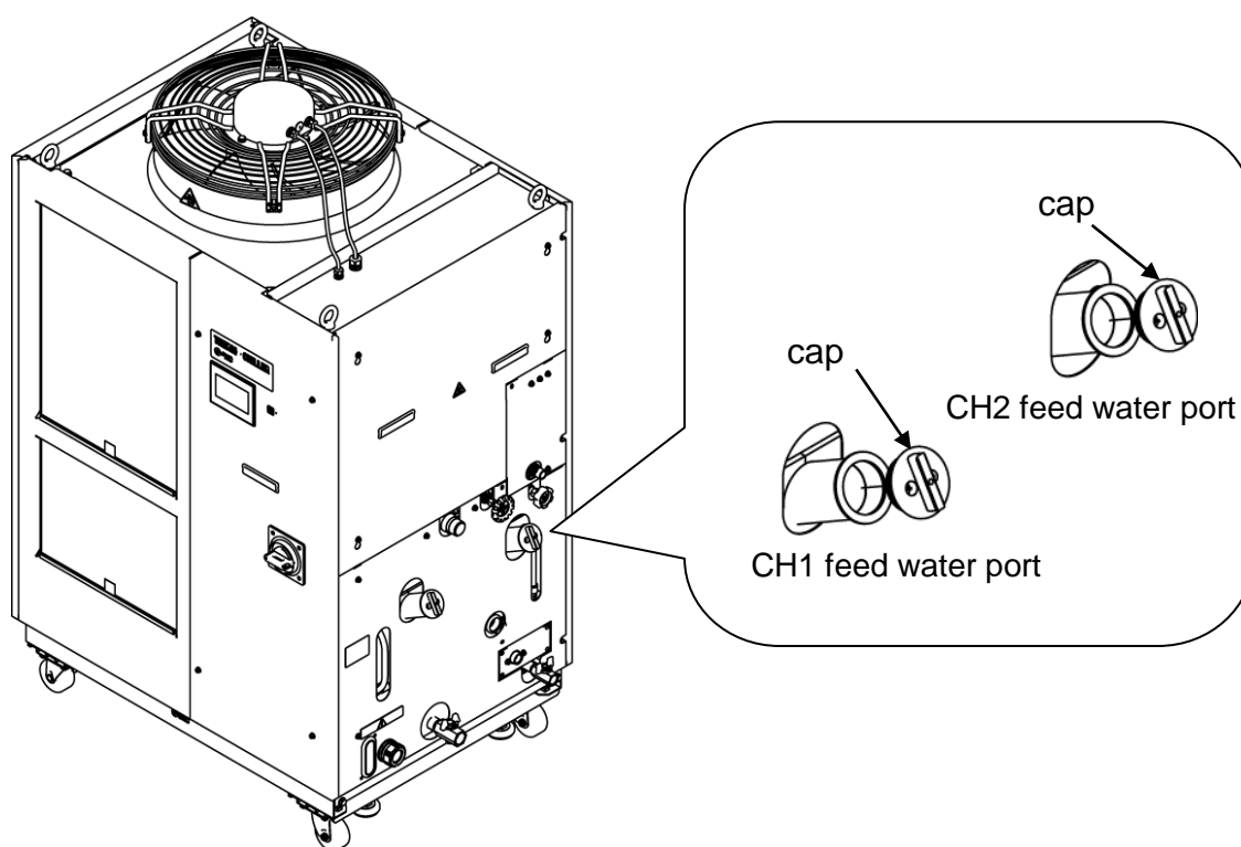
Fig. 3-20 Supplying the fluid to the supply fill port
