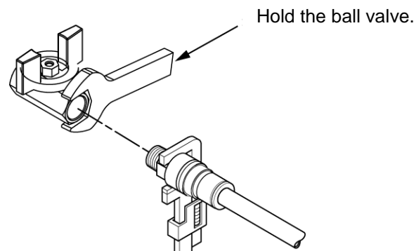
Fig. 3-18 Connection to the drain port
