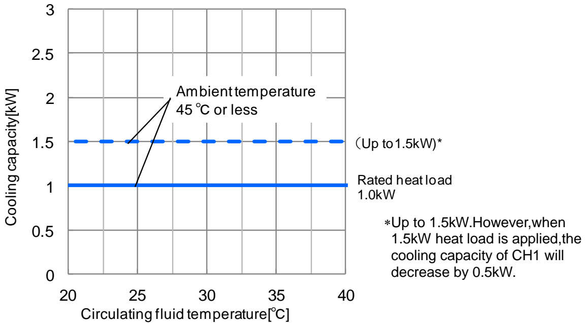
Fig. 8-8 Cooling Capacity (HRL100/200/300-A*-20)
