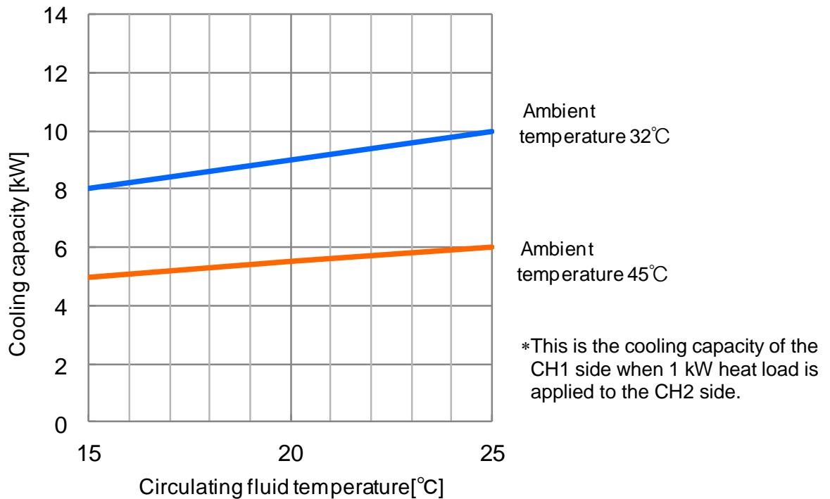
Fig. 8-5 Cooling Capacity (HRL100-A*-20)
