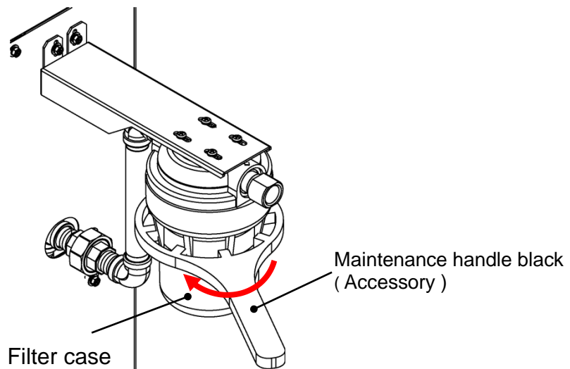
Fig. 3-16 CH2 particle filter case removal
