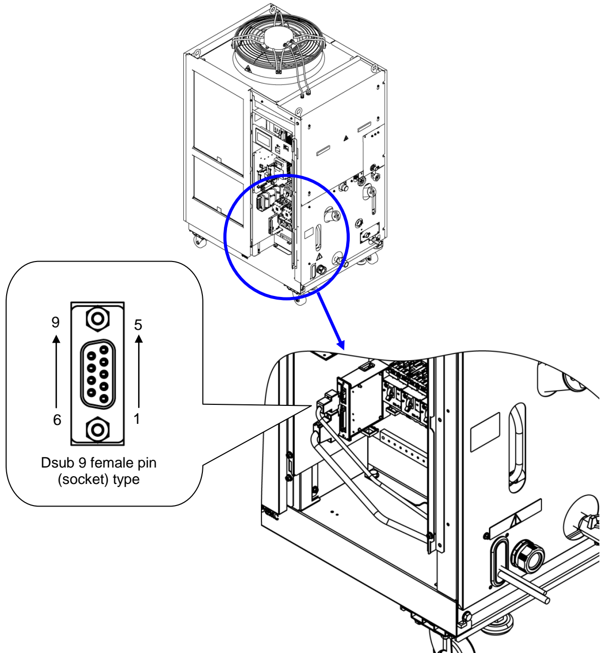
Fig. 3-12 RS-485 communication wiring
