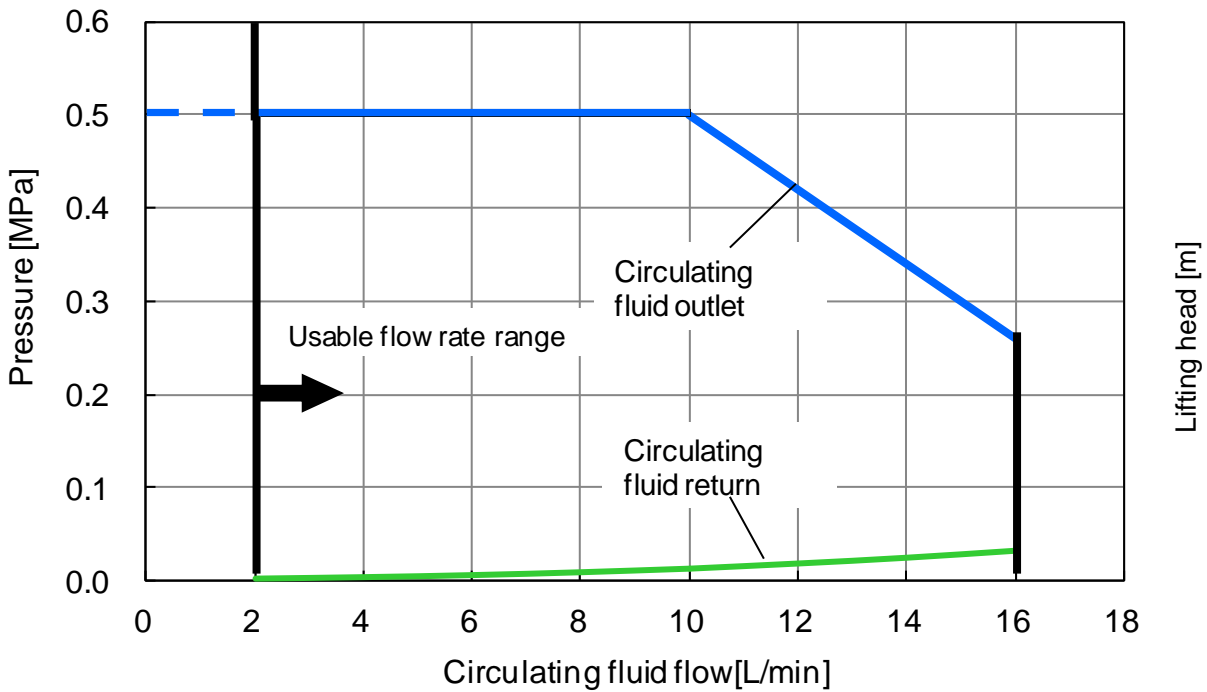
Fig. 8-12 Pump capacity(HRL100/200/300-A*-20 CH2)
