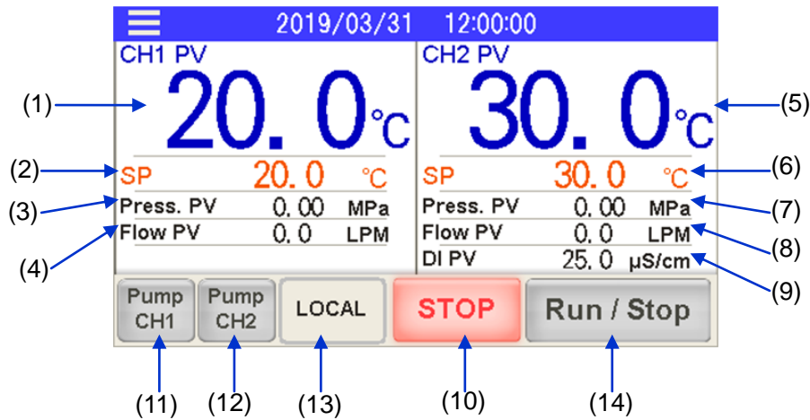
Fig. 4-4 Home screen
