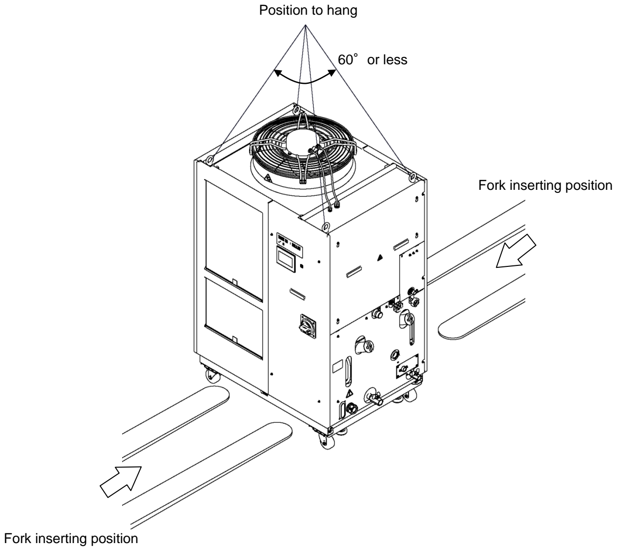
Fig. 3-1 Fork inserting and hanging position (This drawing shows “HRL200-A-20”.)
