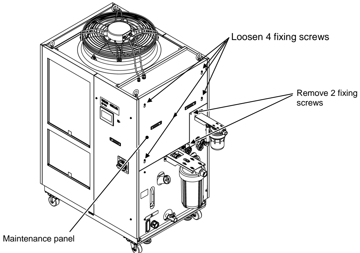
Fig. 7-5 Maintenance panel removal
