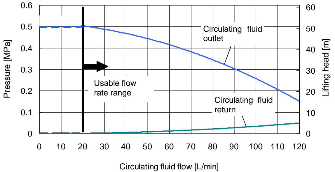
Fig. 8-9 Pump capacity(HRL100-A*-20 CH1)
