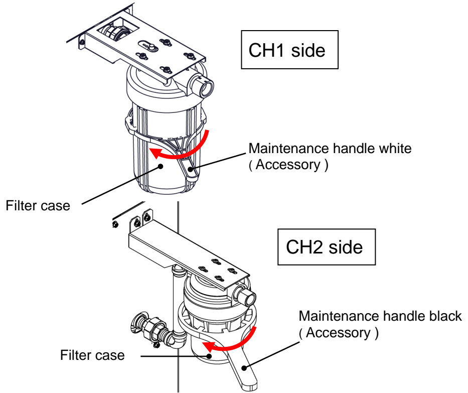
Fig. 7-3 Particle filter removal
