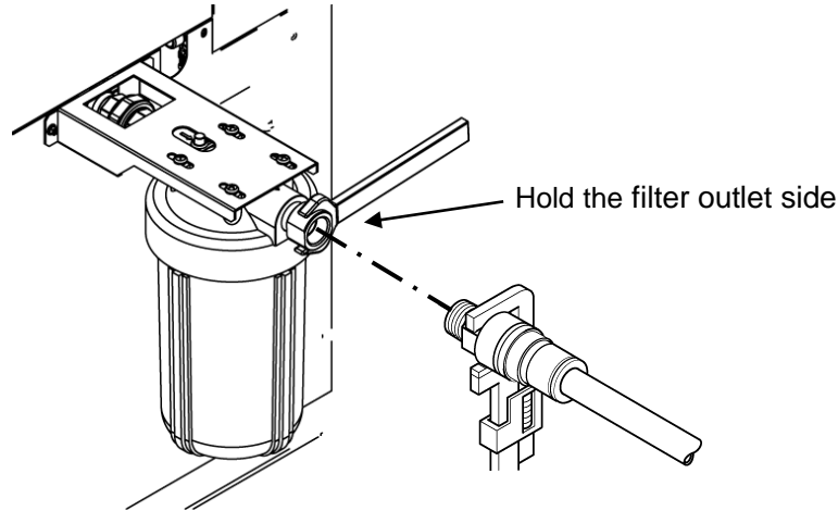
Fig. 3-17 Hold the filter outlet side
