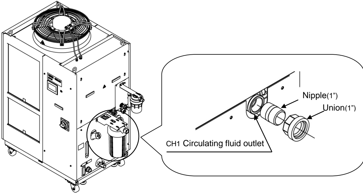
Fig. 3-14 Tightening of piping
