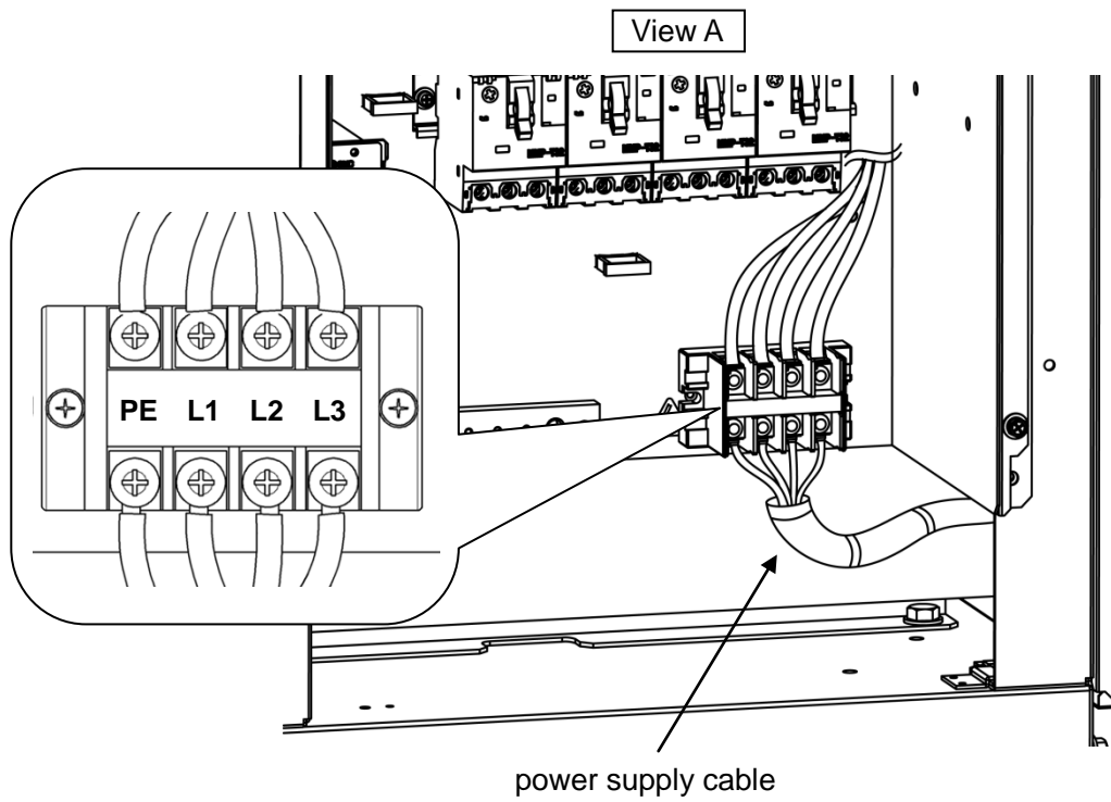
Fig. 3-9 Wiring of power supply cable
