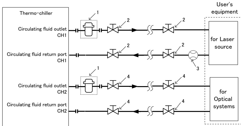
Fig. 3-19 Recommended piping circuit
