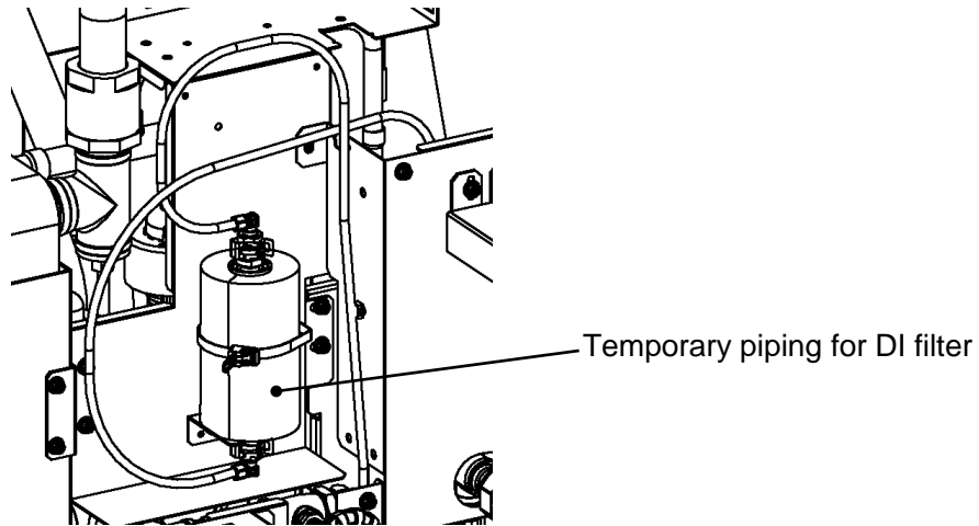
Fig. 7-4 Temporary pipe installation for DI filter
