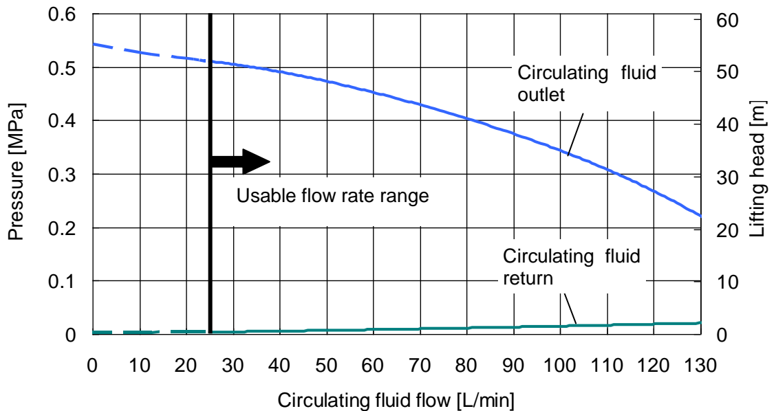
Fig. 8-10 Pump capacity(HRL200-A*-20 CH1)
