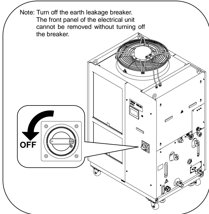
Fig. 3-6 Remove the front panel for the electrical unit
